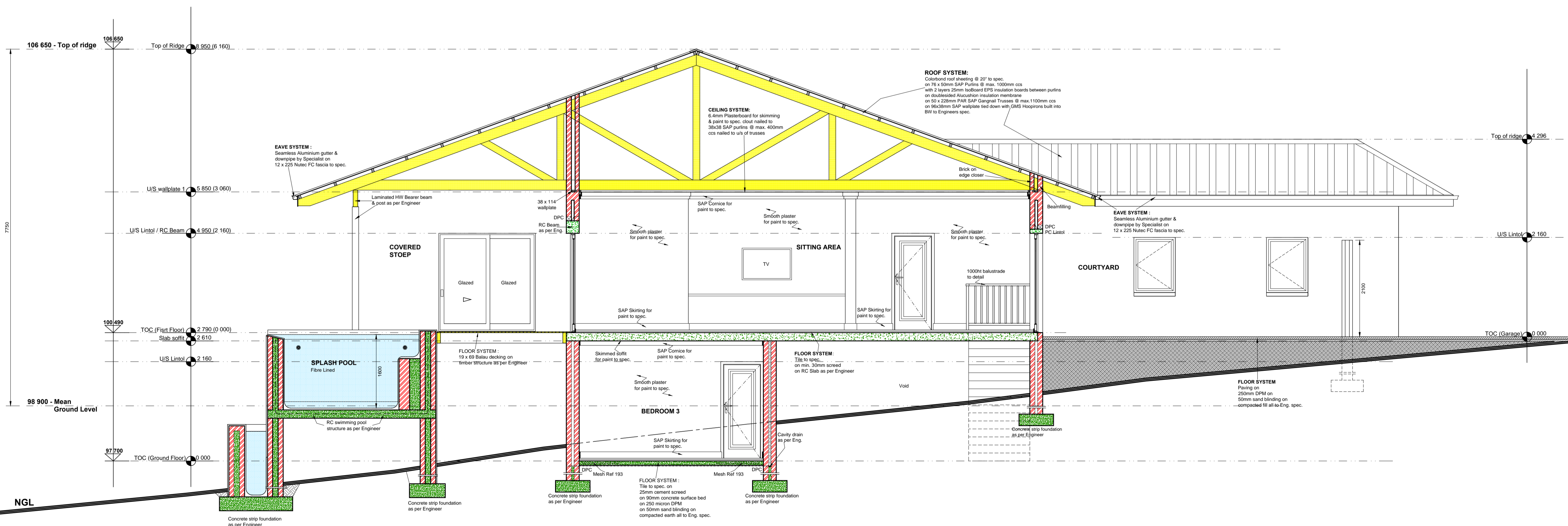
SECTION B-B
